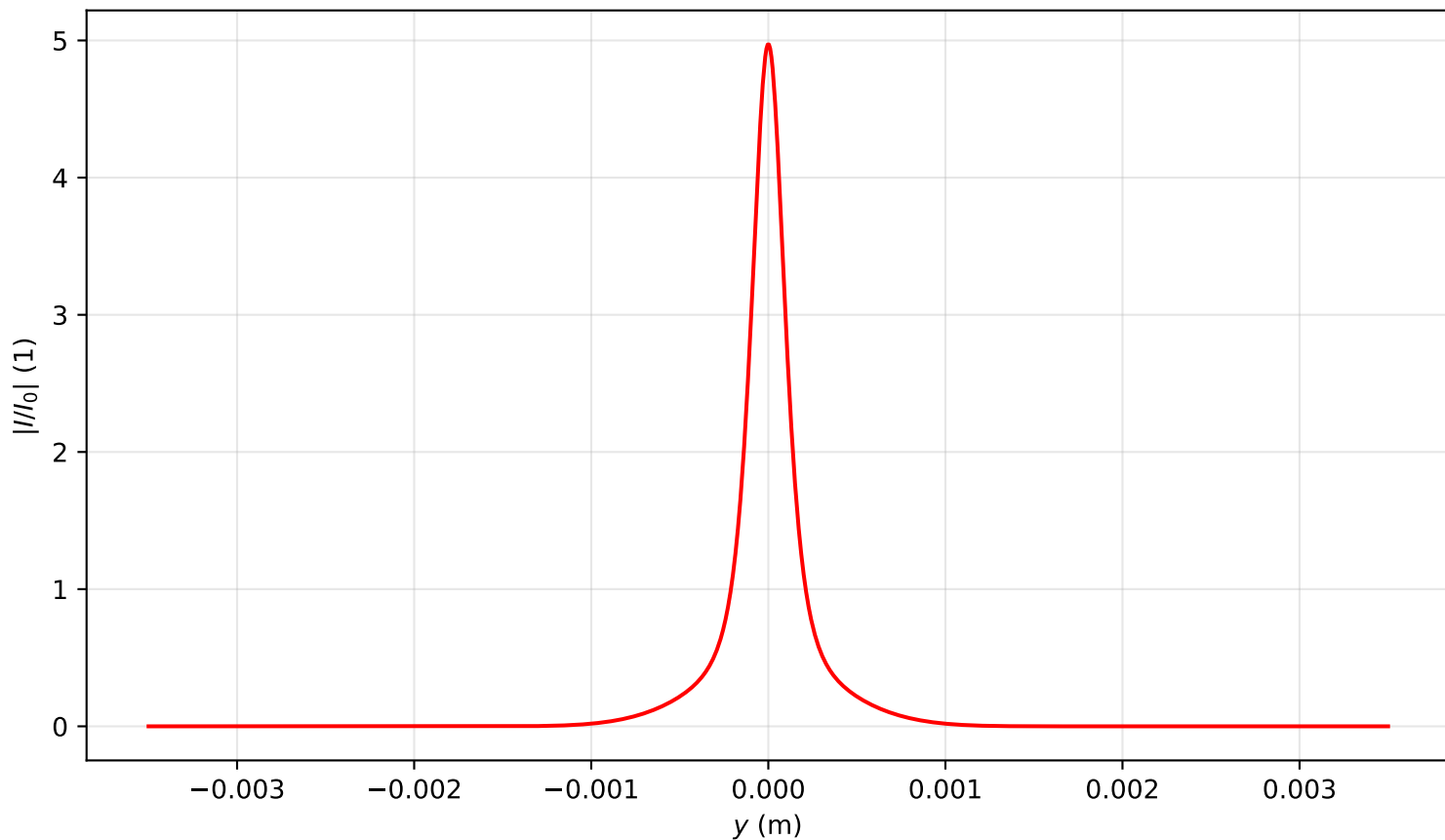
Intensity profile I(x=0, y, z=0.716)/I_0 , P_{in}=2.5P_{cr} , artificial time
